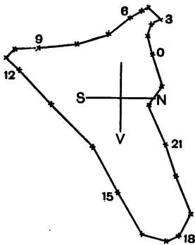
FIG. 13.—KEW DISTURBED DAY VECTOR DIAGRAMS.
